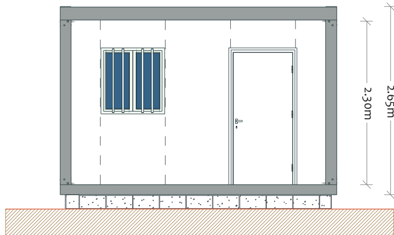
Main Elevation
