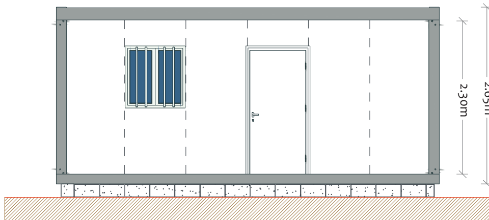
Main Elevation
